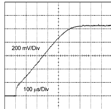
Startup, V_{OUT} = 1.05\text{V} , I_{OUT} = 2\text{A}
