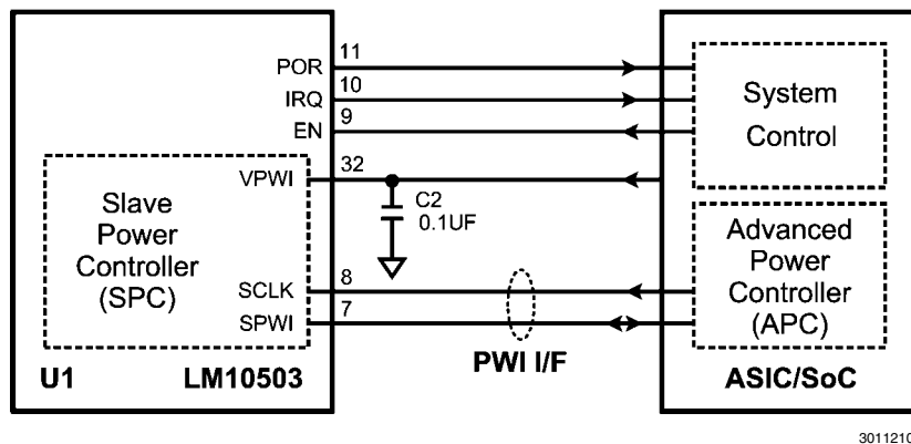
FIGURE 4. PowerWise Interface
