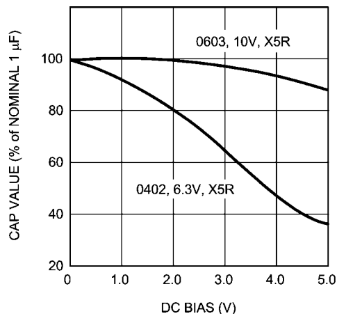
FIGURE 9. Typical Variation in Capacitance vs. DC Bias
