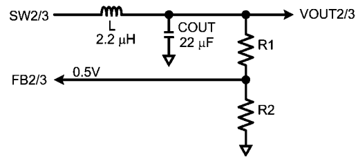
FIGURE 6. Bucks2/3 V_{OUT} Adjust
